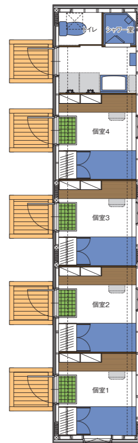
寄宿舍棟 (4P)
